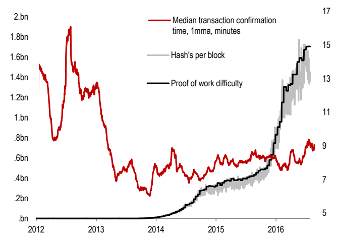
Figure 22: The proof of work difficulty is adjusted such that blocks are added roughly every 10 min
