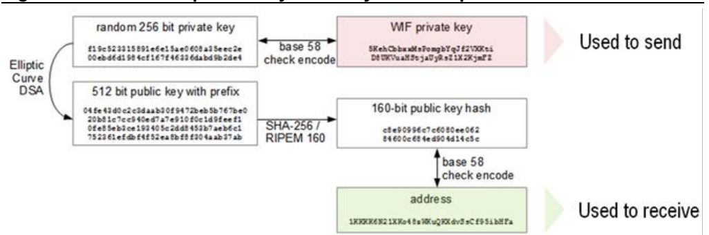
Figure 16: Public and private keys used by bitcoin's protocol
