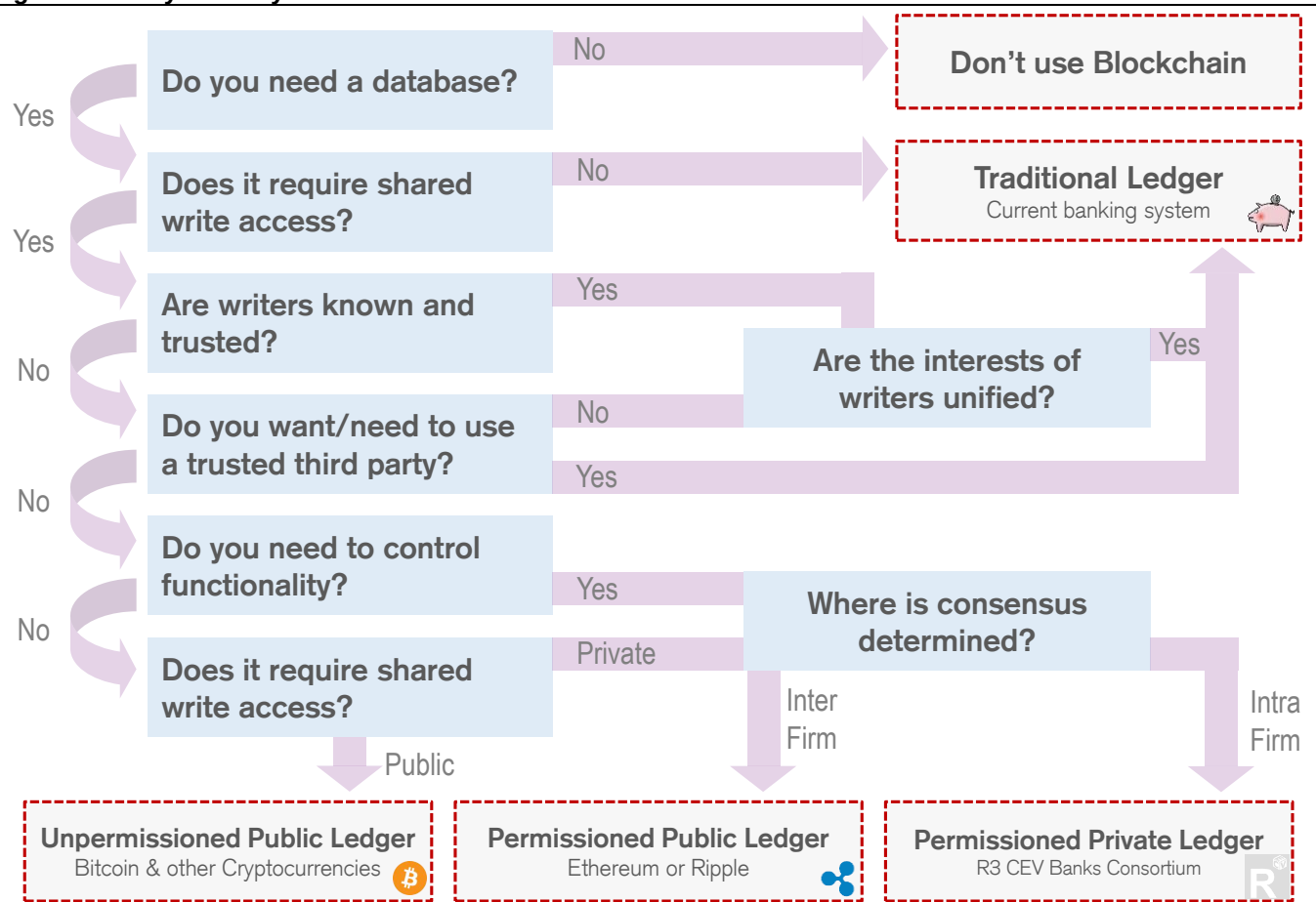
Figure 52: Do you really need a blockchain?
